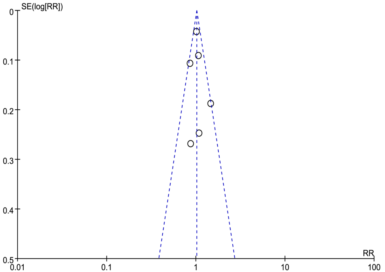
Egger's test
