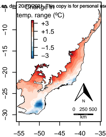
b) Temp. annual range
