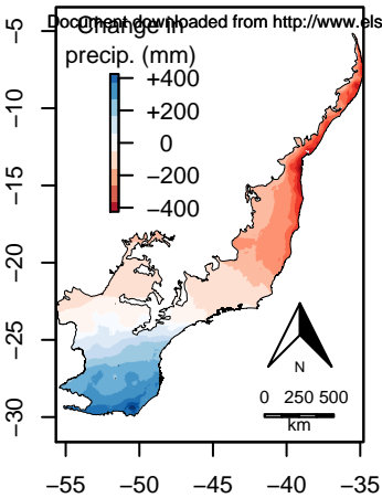
a) Annual precipitation
